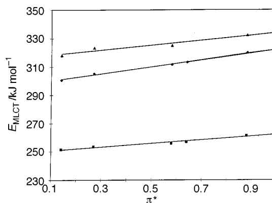
Fig. 3 Energies of MLCT absorption ( E_{\text{MLCT}} ) of (◆) fac -[Re(CO) 3 (dpk)Cl], (▲) cis -[Re(CO) 2 (PPh 3 ) 2 {(C 5 H 4 N) 2 C(O)(OH)}] and (■) cis -[Re(CO) 2 (PPh 3 ) 2 (dpk)Cl] plotted against Taft's \pi^* solvent values in non-chlorinated aliphatic solvents
