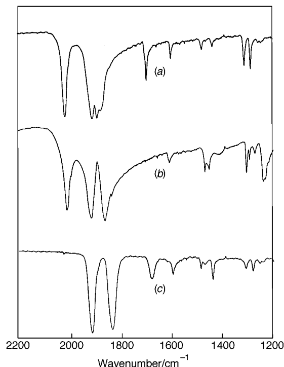
Fig. 1 Infrared spectra of (a) fac -[Re(CO) 3 (dpk)Cl], (b) fac -[Re(CO) 3 {(C 5 H 4 N) 2 C(O)(OH)}] and (c) cis -[Re(CO) 2 (PPh 3 )(dpk)Cl] in KBr pellets
