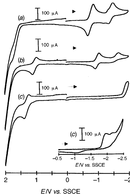
Fig. 5 Cyclic voltammograms of (a) fac -[Re(CO) 3 (dpk)Cl], (b) cis -[Re(CO) 2 (PPh 3 )(dpk)Cl] and (c) fac -[Re(CO) 3 {(C 5 H 4 N) 2 C(O)(OH)}] in dmf solutions (0.1 mol dm -3 NBu 4 PF 6 ) at a glassy carbon working electrode (0.07 cm 2 ) and a scan rate of 400 mV s -1 vs. SSCE
